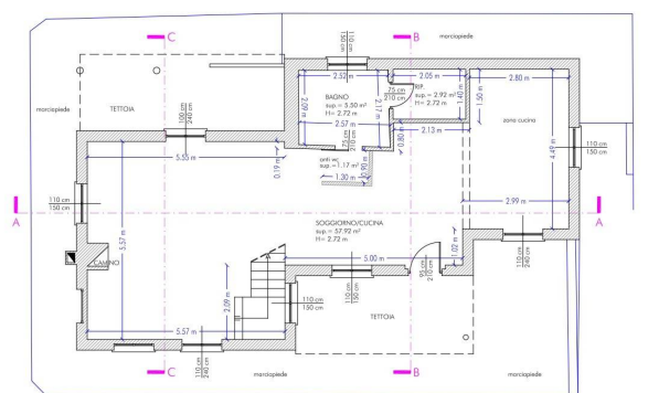
PIANO TERRA scala 1/100
